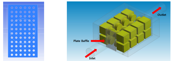
Figure 4. Geometry for the reduction system of exhaust gas with plate baffle.
