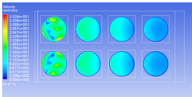
Figure 5. Flow velocity distribution of DOC with plate baffle.
