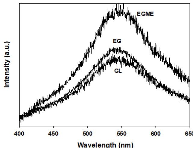
Figure 5. PL spectra of \text{Bi}_2\text{MoO}_6 catalysts prepared using different solvent ( V_{\text{solvent}}/V_{\text{H}_2\text{O}} = 50/50 , synthesis temperature = 180^\circ\text{C} ).
