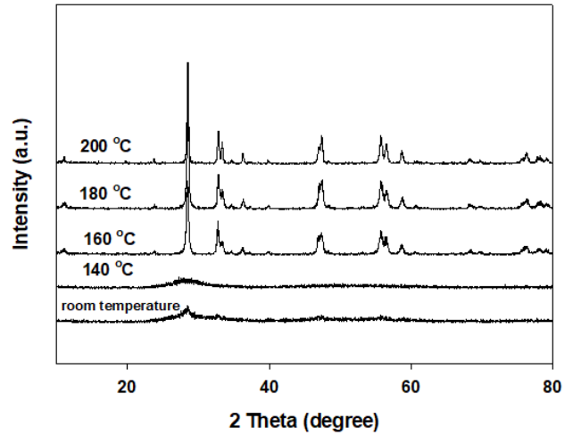
Figure 2. X-ray diffraction patterns of Bi 2 MoO 6 catalysts prepared using different synthesis temperature ( V_{EGME}/V_{H_2O} = 50/50 ).
