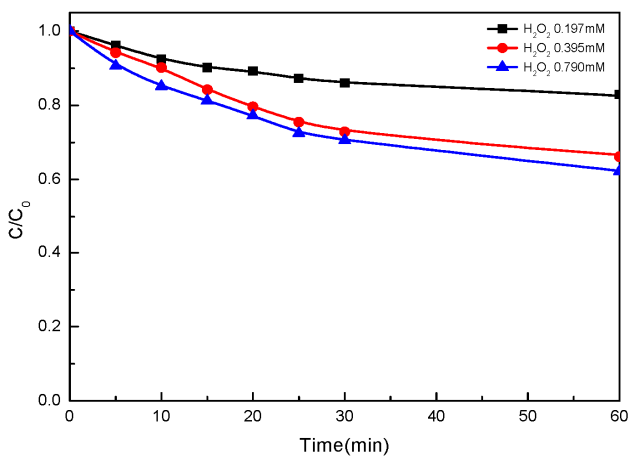
Figure 2. Decomposition of SMX with change of H 2 O 2 concentration at 1 atm, 20 °C and 2 g 10 wt% Cu/Al 2 O 3 .
