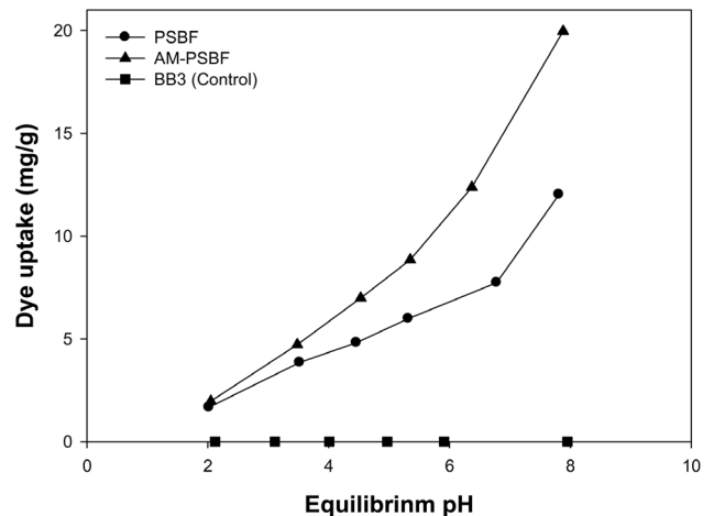
Figure 1. The effect of pH on BB3 adsorption by PSBF and AM-PSBF.
