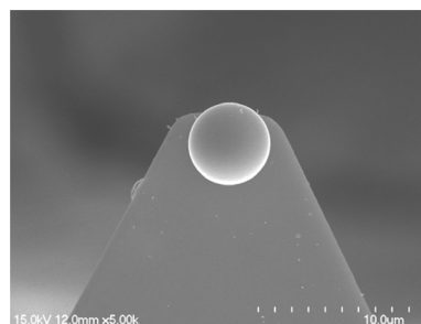
Figure 1. Zirconia sphere-attached-cantilever.
