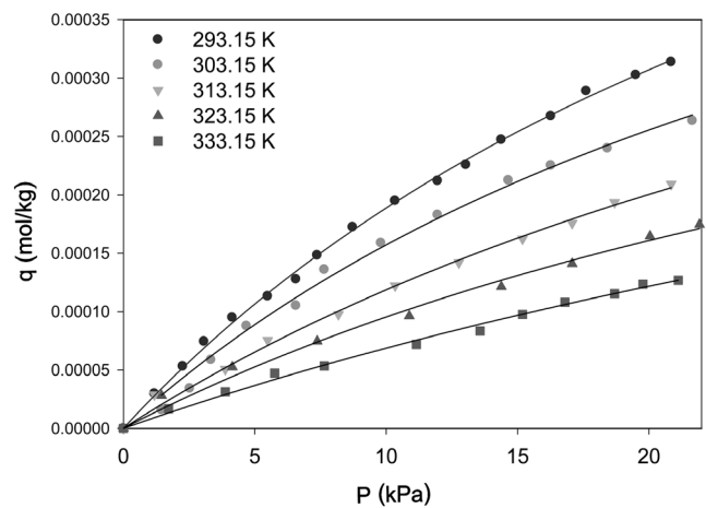
Figure 4. Adsorption isotherms of CF 4 on activated carbon at various temperatures with respect to pressure.
