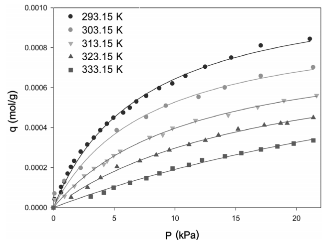
Figure 5. Adsorption isotherms of C 2 F 6 on activated carbon at various temperatures with respect to pressure.
