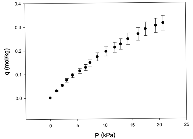
Figure 3. A typical data set of adsorbed amounts with respect to pressure. The error bars are used to imply that the data are scattered and that data reproduction is very hard to accomplish with a new setup of adsorbates.
