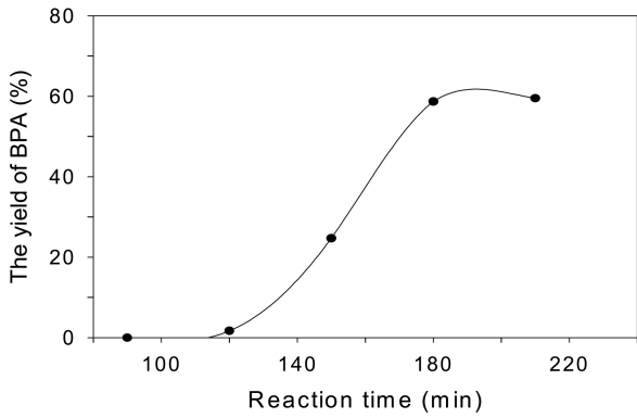
Figure 6. Glycolysis of polycarbonate at 493.15 K.
