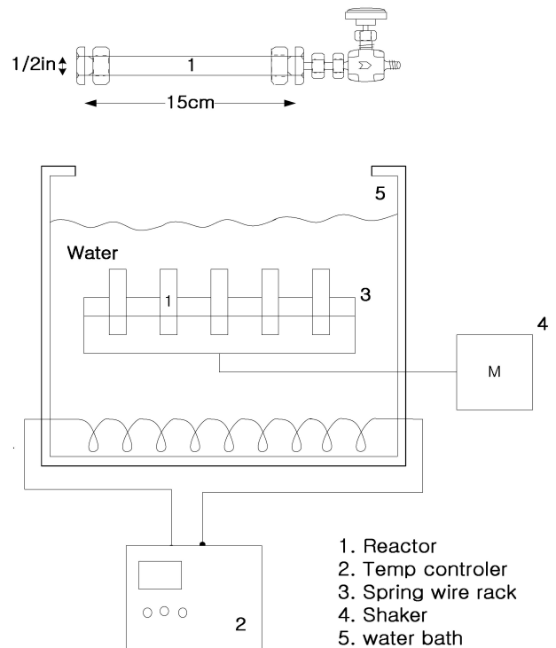
Figure 1. Experimental Apparatus.
