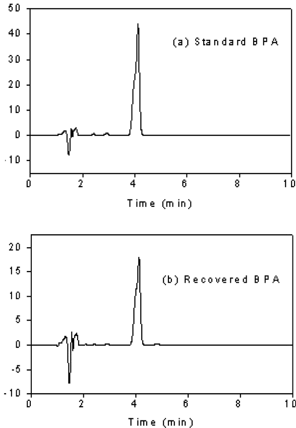
Figure 3. HPLC chromatogram of standard BPA(a) and recovered BPA(b).
