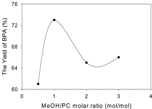
Figure 9. Effect of MeOH/PC molar ratio on the BPA yield.
