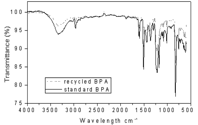
Figure 4. FTIR spectroscopy of standard and recovered BPAs.
