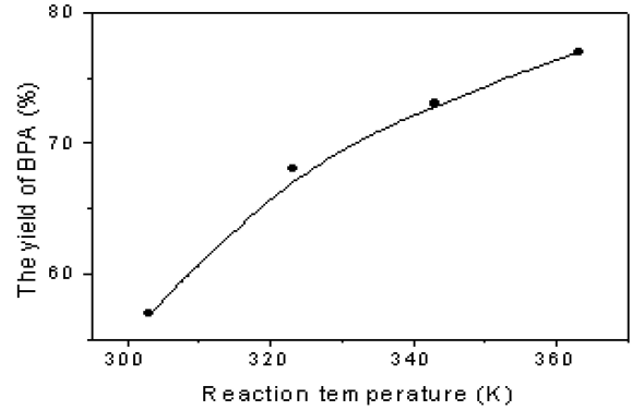
Figure 10. Effect of methanolysis reaction temperature on the BPA yield.
