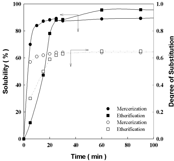
Figure 3. Effects of mercerization and etherification times on solubility and degree of substitution. Reaction temperature = 45°C; NaOH conc. = 40% (w/v); MCA conc. = 30% (w/v).
