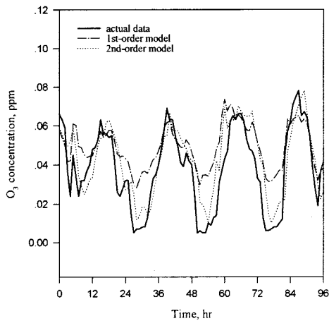
Figure 7. One hour ahead prediction results of O 3 formation using ELS method for the change of model order
