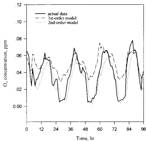
Figure 8. One hour ahead prediction results of O 3 formation using RML method for the change of model order
