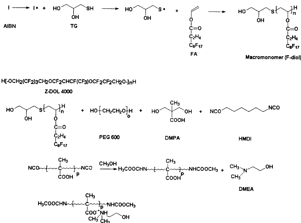
Fig. 1. Synthesis of macromonomer and water-soluble fluorine-containing polyurethane.
