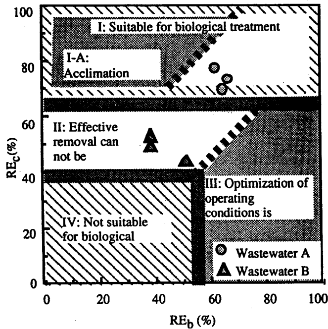
Fig. 7 Biological removal evaluation based on the relationship between DOC removal efficiency observed in BOD5 tests ( RE_b ) and that in the continuous biological treatment experiment with a small scale aerobic submerged biofilter ( RE_c )
